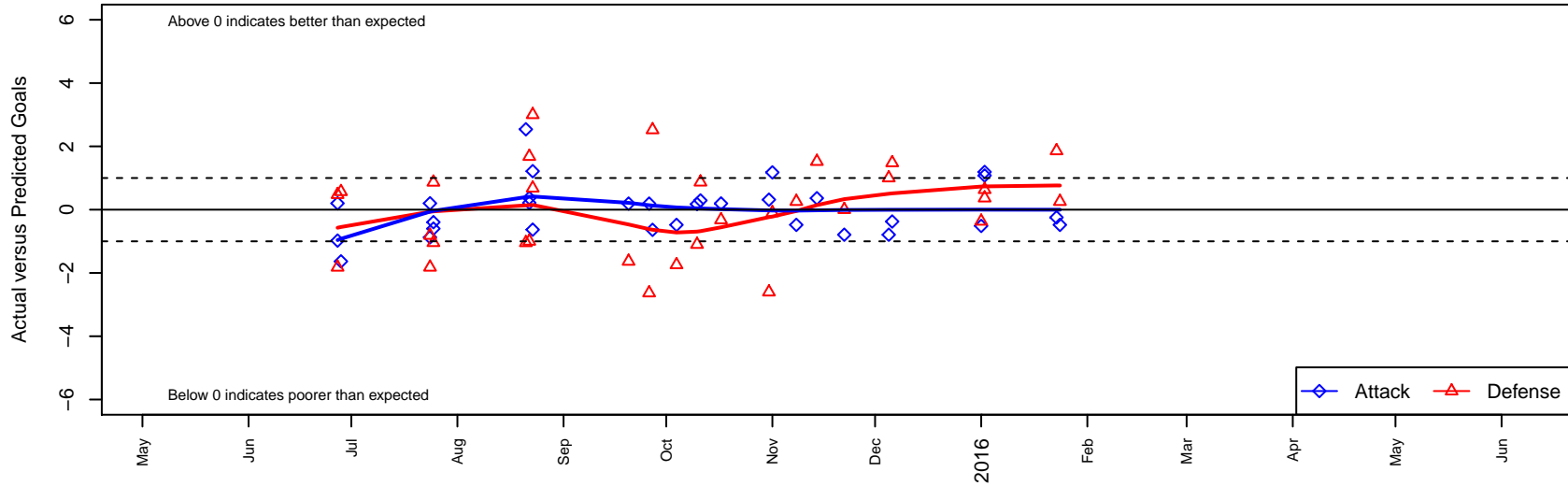
Slammers Orange B98 Dots are actual minus expected GF (blue circles) and GA (red triangles). Blue line is smoothed change in attack strength. Red is smoothed change in defense strength.
